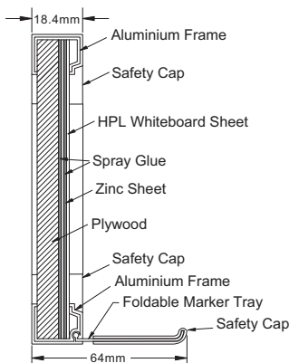
HPL Single Sided Magnetic
