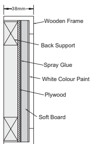
Wooden Frame Cabinet • Soft Notice Board
