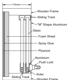
Wooden Frame Cabinet • Foam Notice Board
