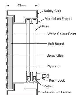
Aluminium Frame Cabinet • Soft Notice Board
