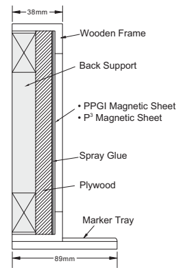
Wooden Frame • PPGI Magnetic Whiteboard • P 3 Magnetic Whiteboard
