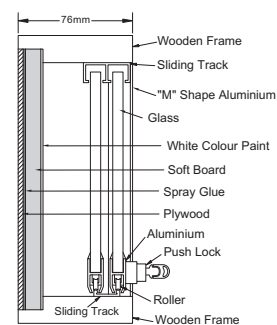
Wooden Frame Cabinet • Soft Notice Board
