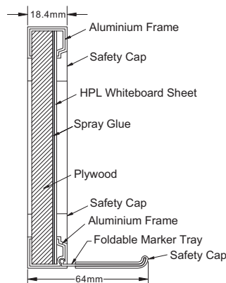
HPL Single Sided Non Magnetic
