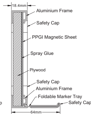
PPGI Single Sided
