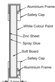
Dual / Combination Board • Soft Notice Board
