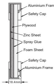
Dual / Combination Board • Foam Notice Board
