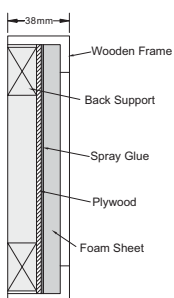
Wooden Frame Cabinet • Foam Notice Board
