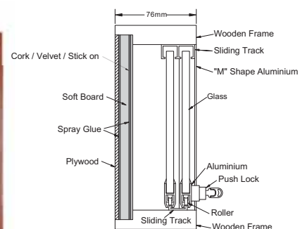
Wooden Frame Cabinet • Cork Notice Board • Velvet Notice Board • Stick on Notice Board
