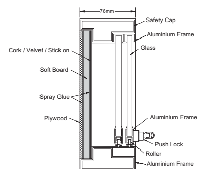
Aluminium Frame Cabinet • Cork Notice Board • Velvet Notice Board • Stick on Notice Board
