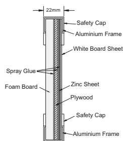
Twin Board with Stand • Foam Notice Board
