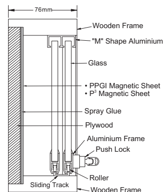
Wooden Frame • PPGI Magnetic Whiteboard • P 3 Magnetic Whiteboard
