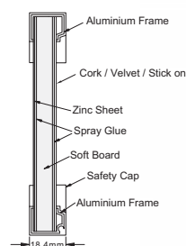
Dual / Combination Board • Cork Notice Board • Velvet Notice Board • Stick on Notice Board
