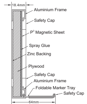
P 3 Single Sided
