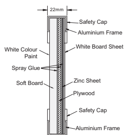
Twin Board with Stand • Soft Notice Board
