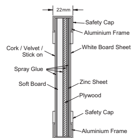
Twin Board with Stand • Cork Notice Board • Velvet Notice Board • Stick on Notice Board
