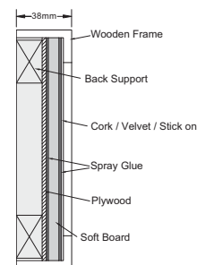
Wooden Frame Cabinet • Cork Notice Board • Velvet Notice Board • Stick on Notice Board
