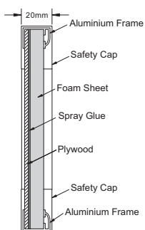
Aluminium Frame • Foam Notice Board
