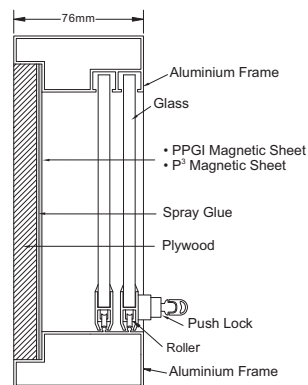
Aluminium Frame Cabinet • PPGI Magnetic Whiteboard • P³ Magnetic Whiteboard
