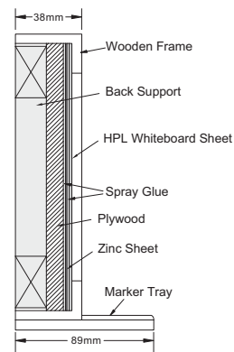
Wooden Frame • HPL Magnetic Whiteboard
