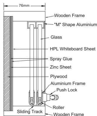
Wooden Frame • HPL Magnetic Whiteboard
