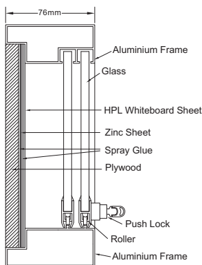
Aluminium Frame Cabinet • HPL Magnetic Whiteboard
