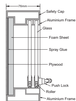
Aluminium Frame Cabinet • Foam Notice Board
